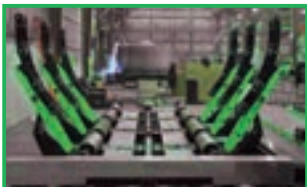
Hydraulic alignment jacking system to align and pull vessel sections together.
