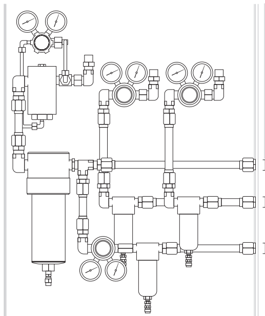
LaserStar RFP Regulator Filter Panels (RFP)
