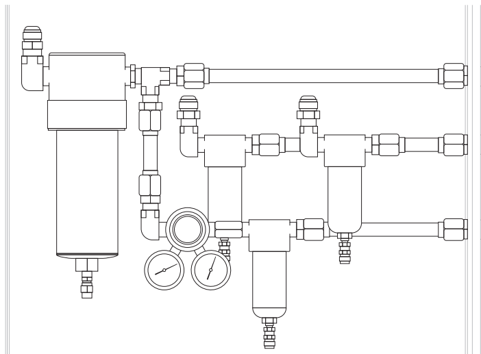
LaserStar Filter Panel (FP)
